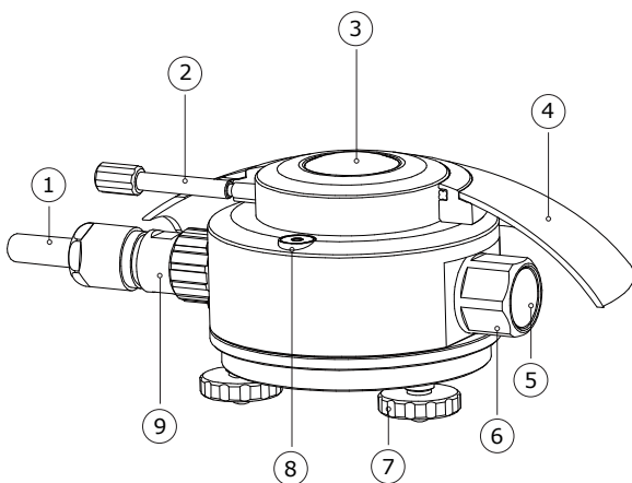
Figure 2 overview of GEO-IR20 pyrgeometer: (1) cable, (2) fixation of sun screen, (3) dome with solar blind filter, (4) sun screen, (5) humidity indicator, (6) desiccant holder, (7) levelling feet, (8) bubble level, (9) connector
